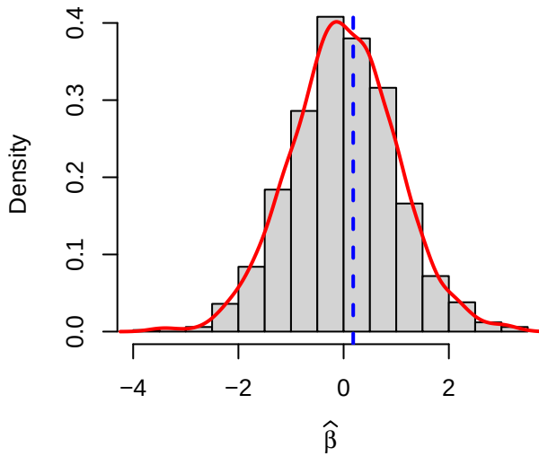
Case 9 (transformed data): \alpha = 1.0 , \beta = 1.2 , b = 1.0 , \rho = 0.8
