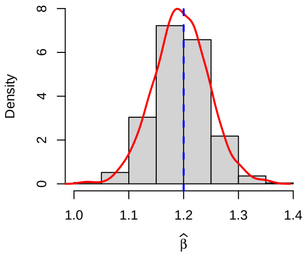
Case 9: \alpha = 1.0 , \beta = 1.2 , b = 1.0 , \rho = 0.8
