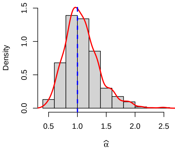
Case 9: \alpha = 1.0 , \beta = 1.2 , b = 1.0 , \rho = 0.8
