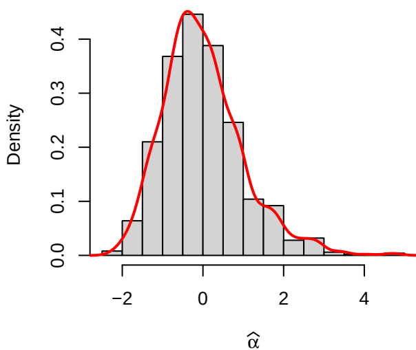
Case 9 (transformed and normalized data): \alpha = 1.0 , \beta = 1.2 , b = 1.0 , \rho = 0.8
