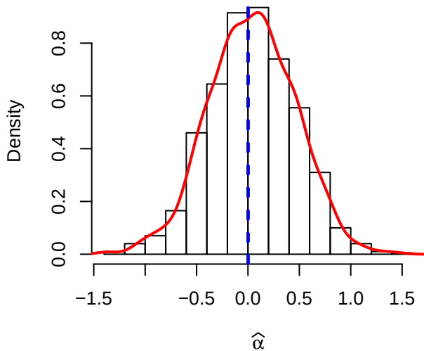
Case 3 (transformed data): \alpha = 1.0 , \beta = 1.0 , b = 1.0 , \rho = 0.8
