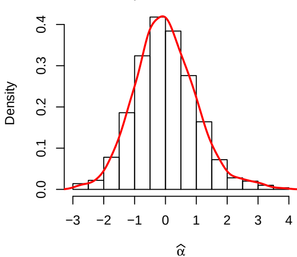
Case 8 (transformed and normalized data): \alpha = 1.0 , \beta = 1.2 , b = 1.0 , \rho = 0.5
