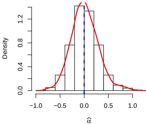
Case 8 (transformed data): \alpha= 1.0 , \beta= 1.2 , b= 1.0 , \rho= 0.5
