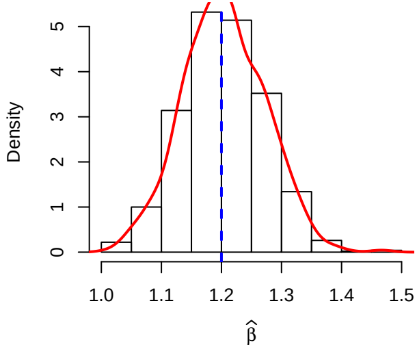
Case 8 (original data): \alpha= 1.0 , \beta= 1.2 , b= 1.0 , \rho= 0.5
