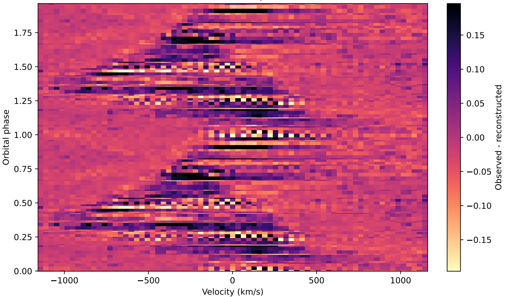
Residual trailed spectra
