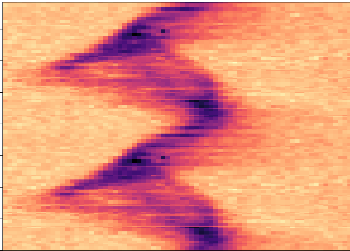
V834 Cen He II 4686 trailed spectra
