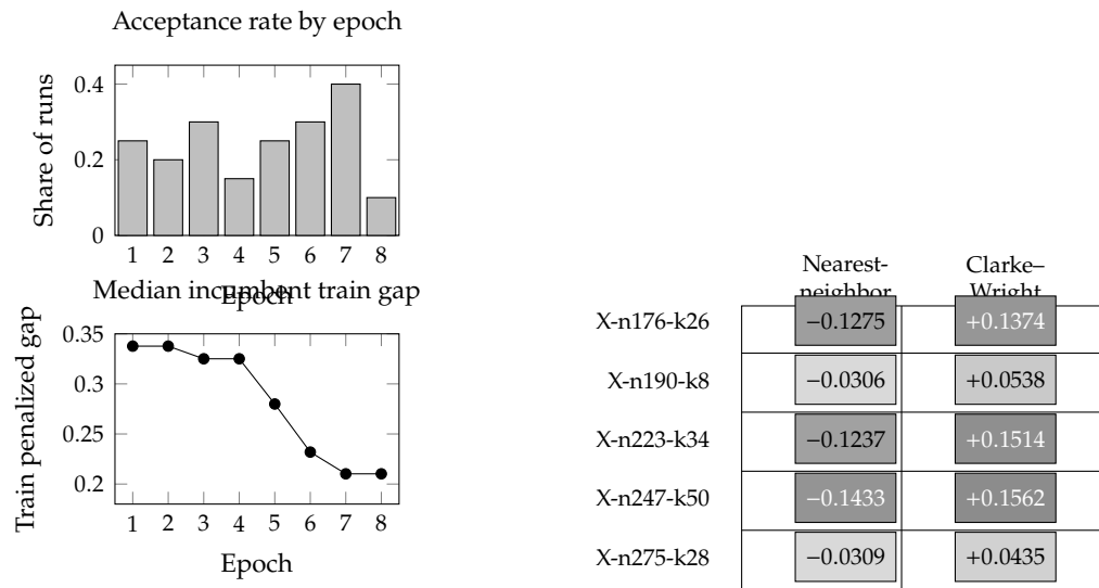
Figure 6.2: Additional diagnostics for the official phase-9 solver-evolution campaign. The left panels use all twenty official runs and track the accepted-update rate by epoch together with the median incumbent train penalized gap, starting from the shared nearest-neighbor constructive incumbent. The right panel aggregates the five held-out X instances across the same twenty runs. Solver evolution beats nearest-neighbor on every held-out instance, but it trails Clarke-Wright on every held-out instance. Darker cells mark larger absolute differences, and negative values favor solver evolution.
