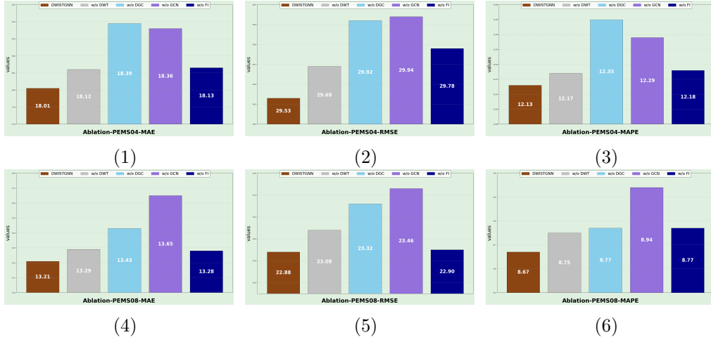
Figure 7: Histogram of Ablation Study
