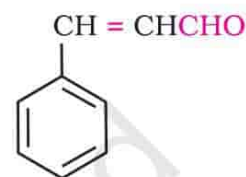
Cinnamaldehyde
