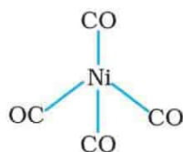
\text{Ni(CO)}_4 Tetrahedral
