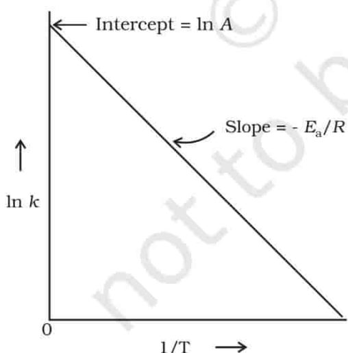
Fig. 3.10: A plot between \ln k and 1/T
