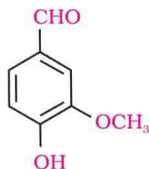
Vanillin
