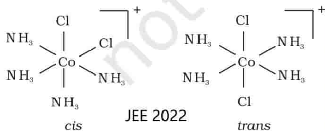
Fig. 5.3: Geometrical isomers ( cis and trans ) of [\text{Co}(\text{NH}_3)_4\text{Cl}_2]^+
