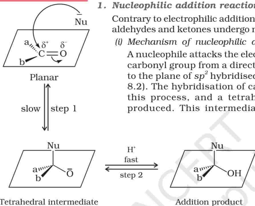
Fig.8.2: Nucleophilic attack on carbonyl carbon
