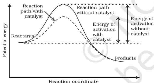
Fig. 3.11: Effect of catalyst on activation energy
