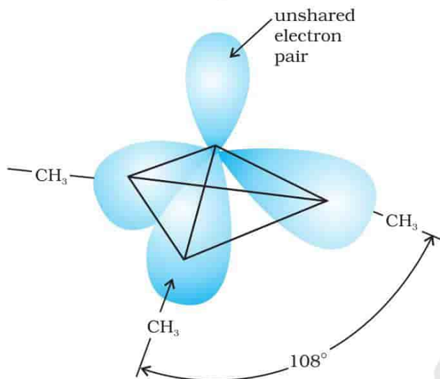
Fig. 9.1 Pyramidal shape of trimethylamine
