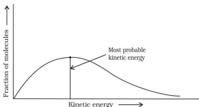
Fig. 3.8: Distribution curve showing energies among gaseous molecules
