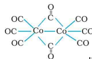
[\text{Co}_2(\text{CO})_8]
