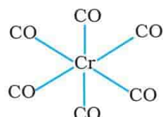
\text{Cr(CO)}_6 Octahedral
