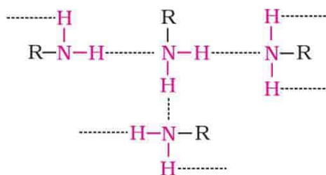
Fig. 9.2 Intermolecular hydrogen bonding in primary amines
