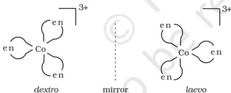
Fig.5.6: Optical isomers (d and l) of [\text{Co}(\text{en})_3]^{3+}
