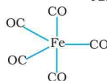
\text{Fe(CO)}_5 Trigonal bipyramidal
