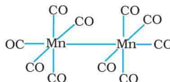
[\text{Mn}_2(\text{CO})_{10}]
