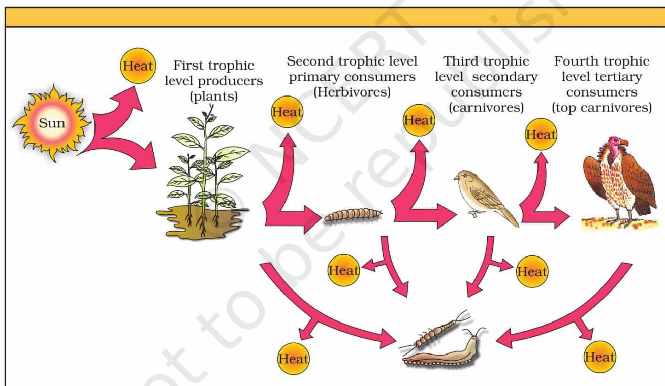
Figure 12.3 Energy flow through different trophic levels
