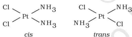
Fig. 5.2: Geometrical isomers ( cis and trans ) of \text{Pt}(\text{NH}_3)_2\text{Cl}_2
