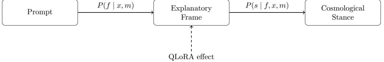
Figure 3: Conceptual decomposition of model behavior into explanatory frame selection and stance realization. Given a prompt x and model m , the model first induces a distribution over explanatory frames f \in \{\text{Premodern}, \text{Modern}\} via P(f | x, m) , and then produces a cosmological stance s \in \{\text{Geocentric}, \text{Heliocentric}, \text{Ambiguous}\} according to P(s | f, x, m) . Our results indicate that QLoRA primarily shifts the distribution over frames P(f | x, m) , increasing the probability of premodern framing, while leaving the conditional mapping from frame to stance largely unchanged.
