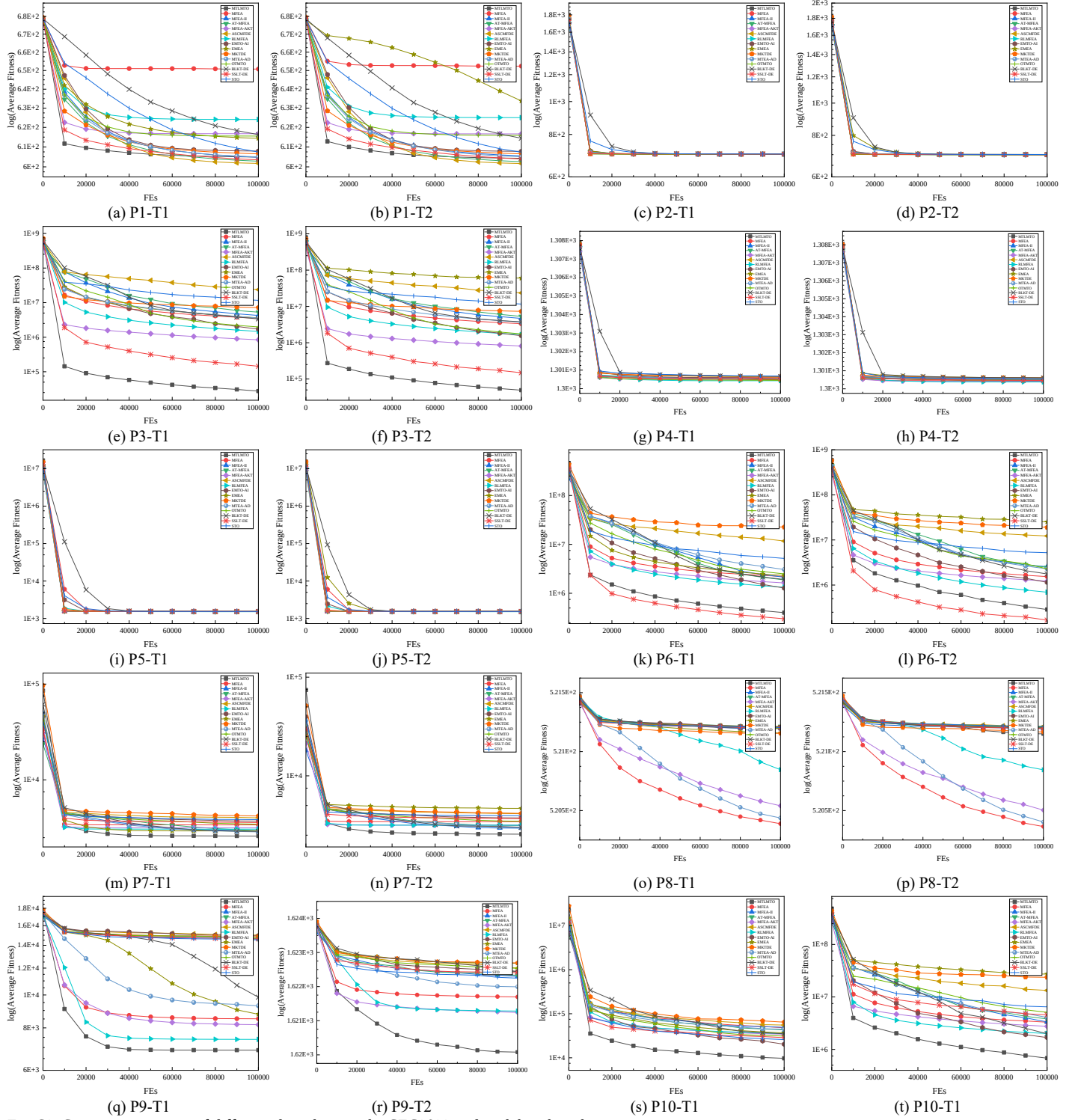
Fig. S2. Convergence curves of different algorithms on the CEC2022 multitask benchmark.
