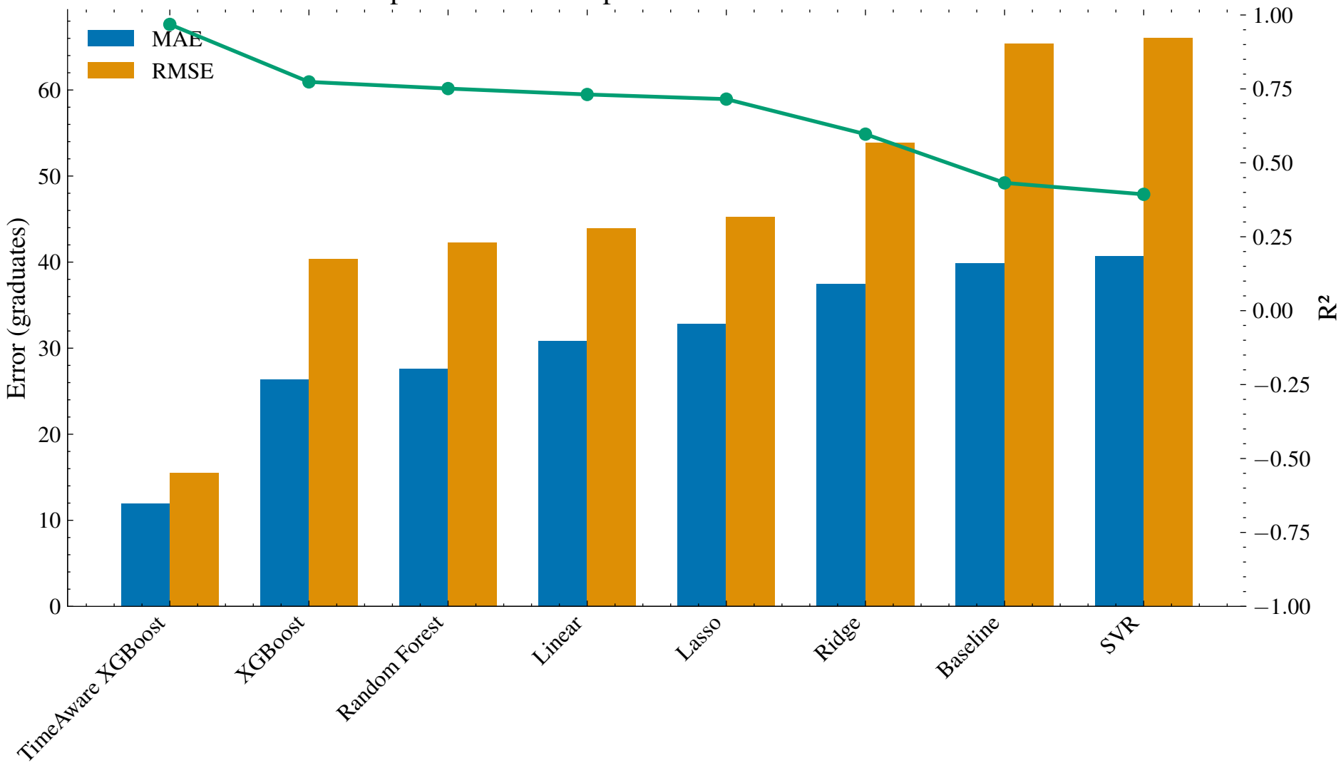
Model performance comparison — MAE / RMSE with R^2
