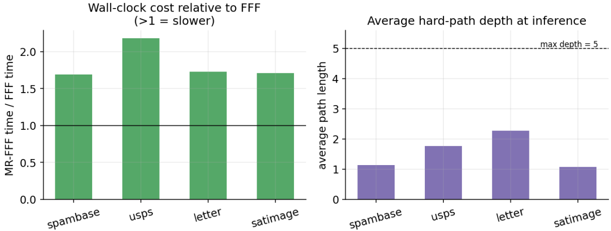
Figure 6: Left: MR-FFF inference time divided by FFF time. Right: average length of MR-FFF paths
