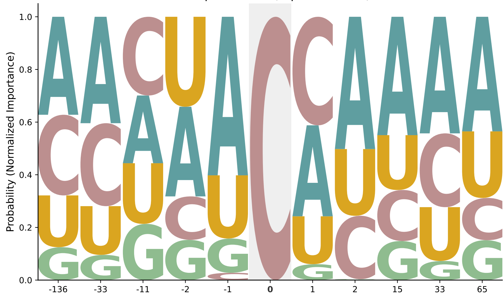
Cm: Spatial Motif (Top 10 Context)
