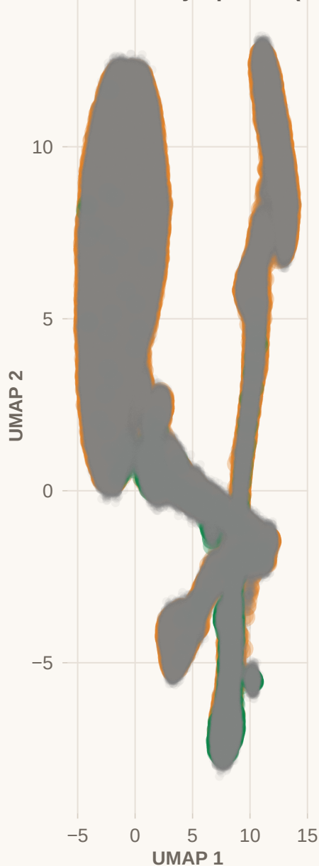
Human Joint UMAP by Class (attention_output)
