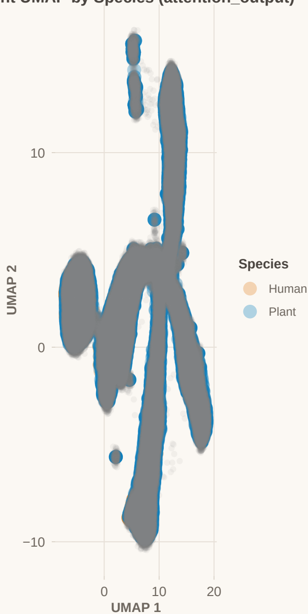
Joint UMAP by Species (attention_output)
