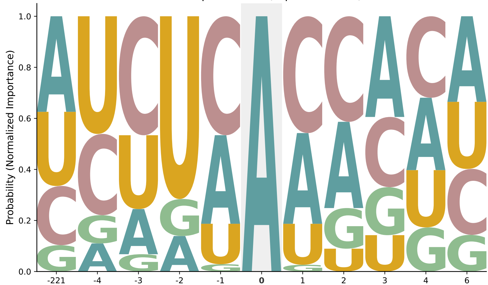
m1A: Spatial Motif (Top 10 Context)
