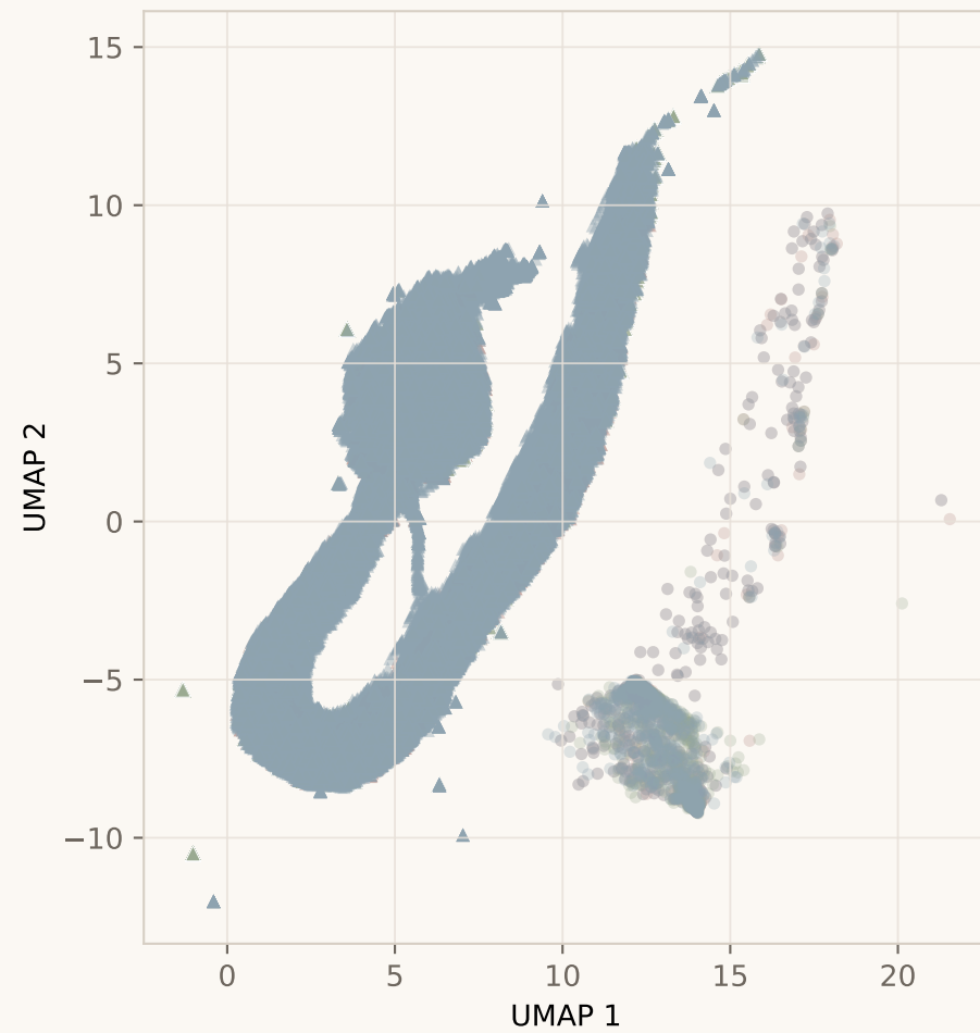
1-shot
