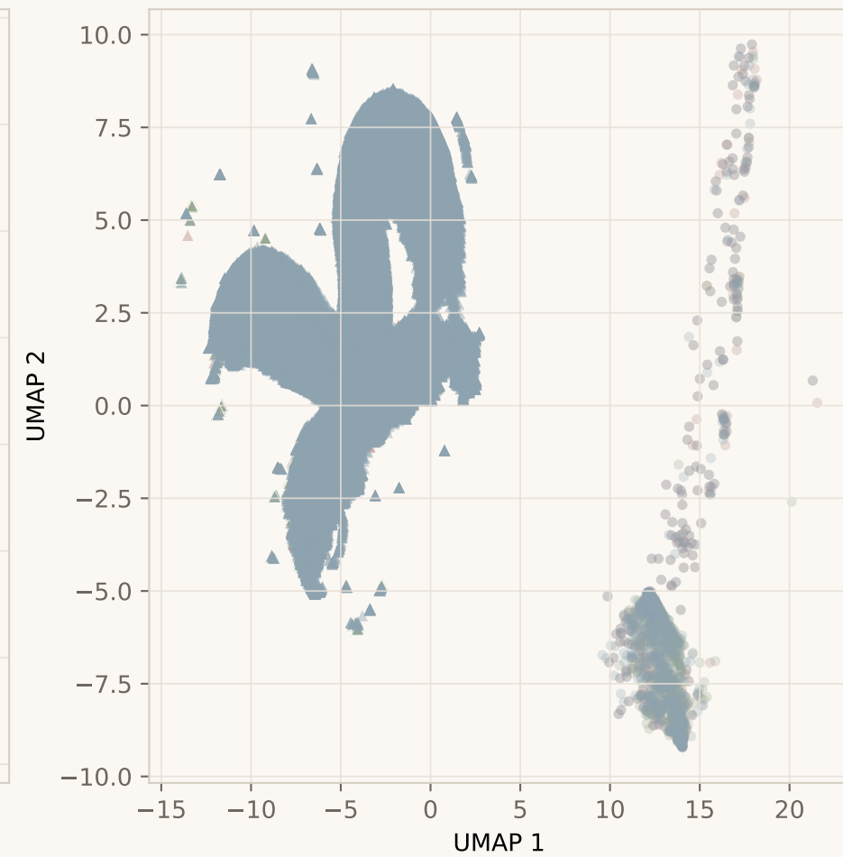
10-shot
