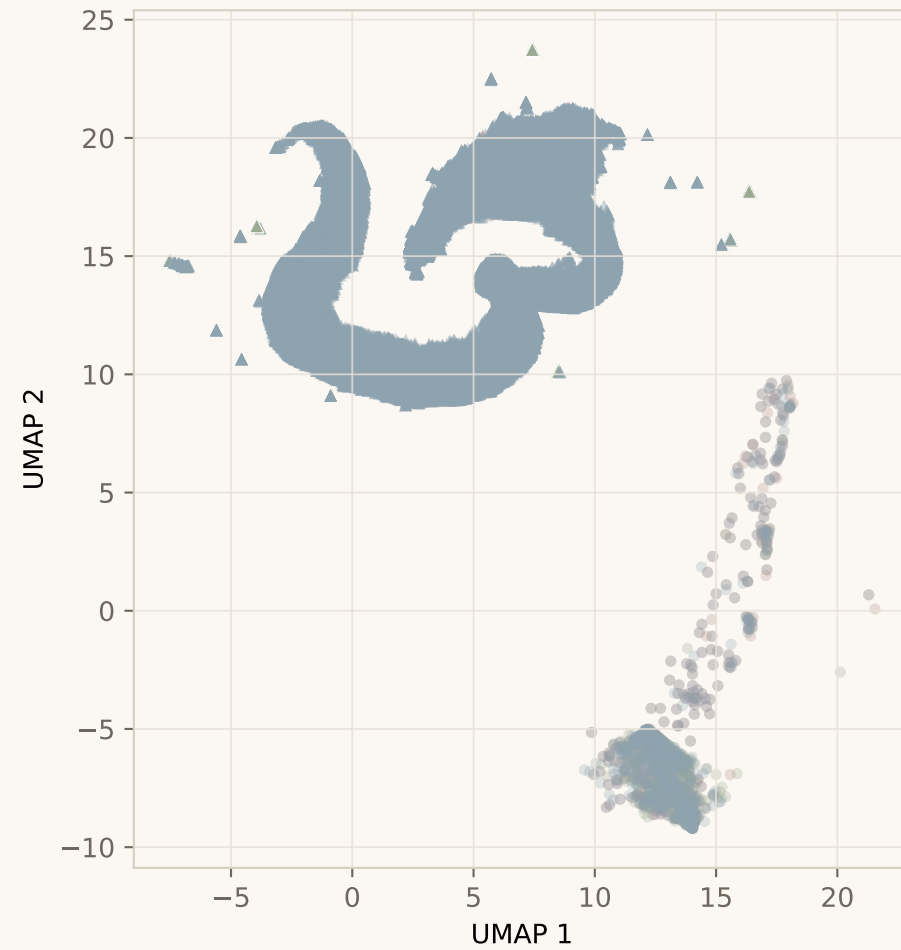
5-shot
