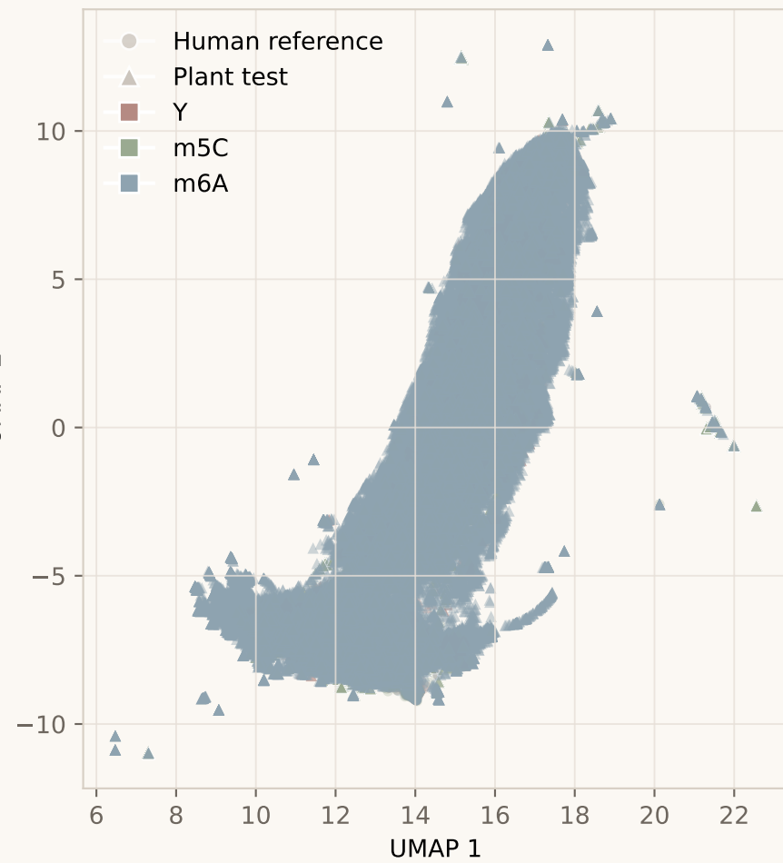
0-shot
