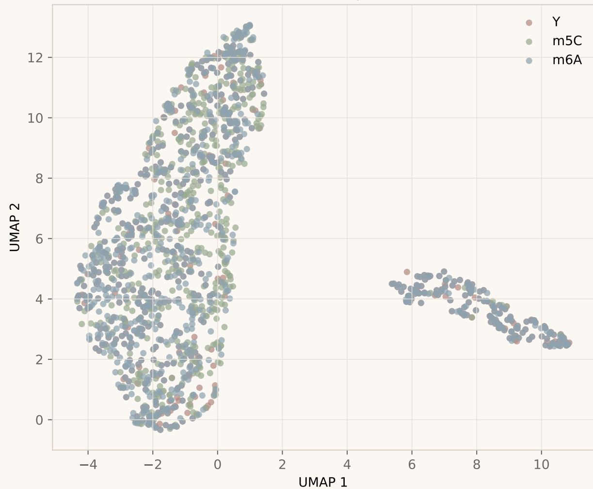
Human UMAP by Class
