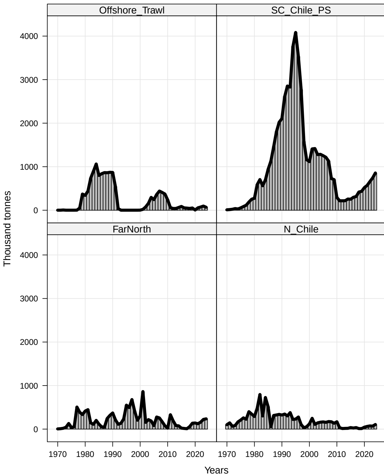
Predicted and observed catches by fleet Observed Predicted
