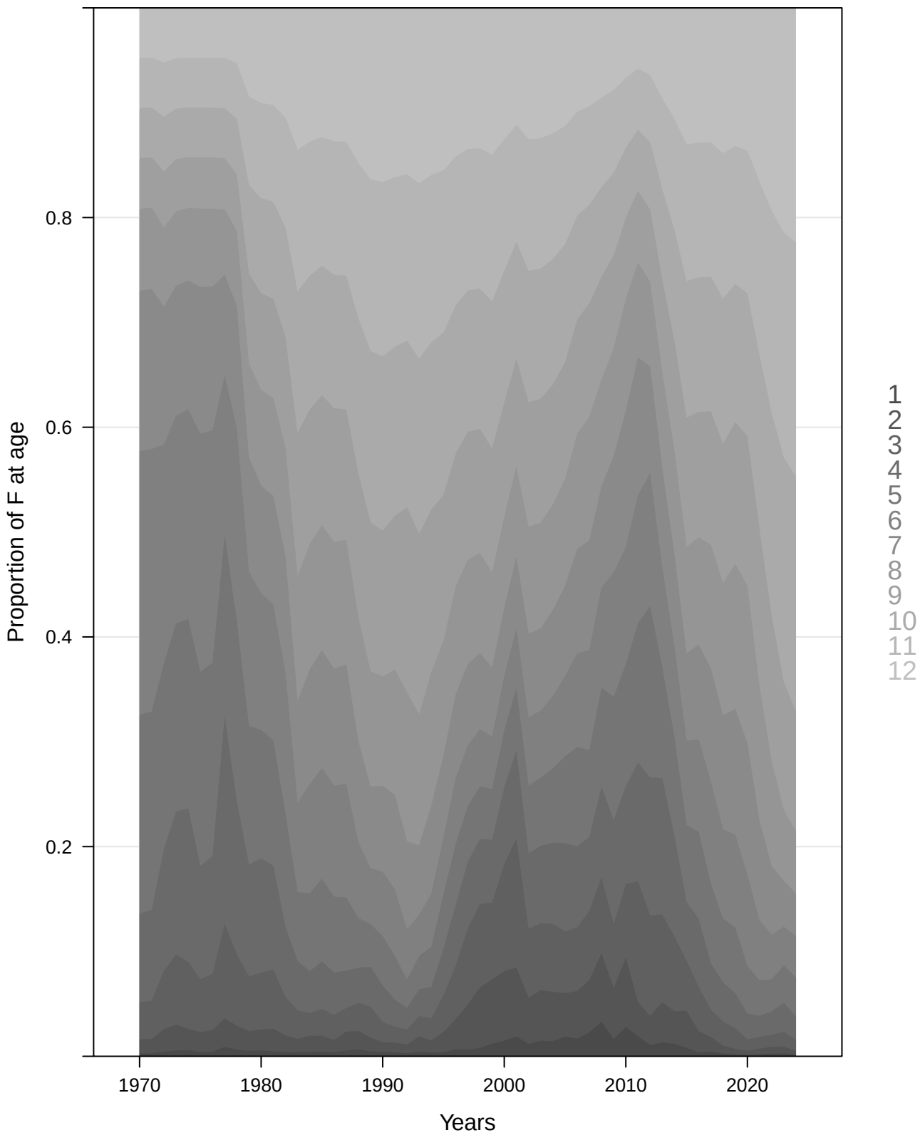
F proportion at age
