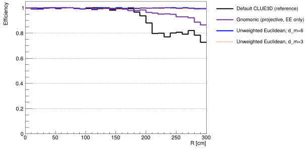
(a) Photon reconstruction efficiency.
