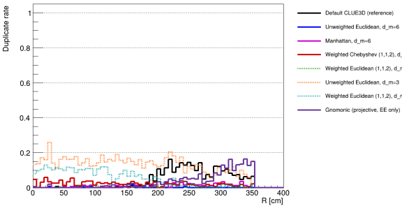
(a) Signal-photon duplicates versus truth displacement.
