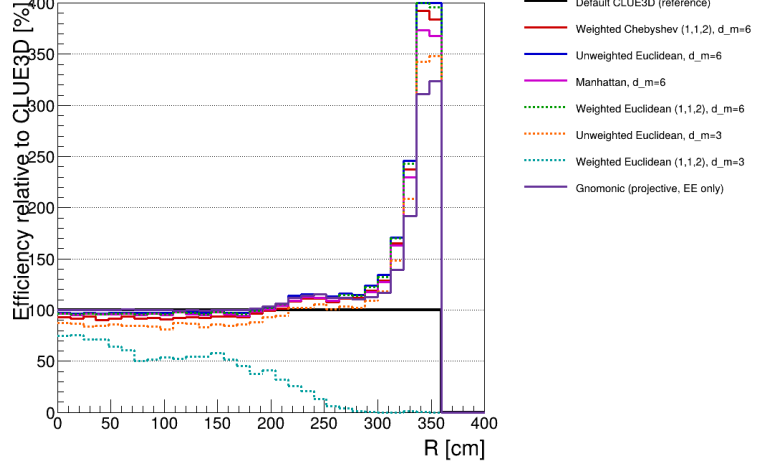
Figure 16: Single-photon efficiency without pileup for the exploratory CLUEstering configurations. The right panel shows 100\epsilon/\epsilon_{\text{CLUE3D}} ; 100 % denotes equal efficiency.
