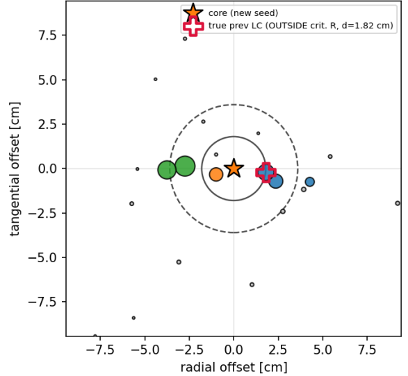
Figure 8: A neighbourhood in the full projected coordinates for the R \simeq 297 cm event previously shown in Fig. 7. The star marks the layer-51 core of a new fragment, and circles the 1.8 cm and 3.6 cm distances.
