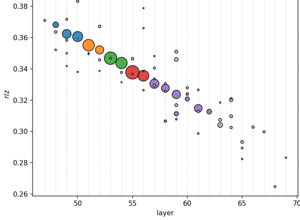
Figure 7: A single photon at R \simeq 297 cm split into five reconstructed Tracksters, shown as r/z versus layer index. Colour identifies the reconstructed Trackster and marker size the energy; grey markers are outliers. The layer index follows the TICL convention, in which positive-endcap layers are offset to accommodate the negative endcap. r/z is not constant.
