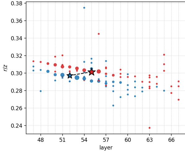
Figure 13: An actual cross-shower nearest-higher link for photons separated by s = 4 cm at R \simeq 131 cm, shown as r/z versus layer. Blue marks the simulated truth shower A and red the simulated truth shower B , rather than reconstructed Trackster membership; the dashed line is the recorded nearest-higher hop from B 's highlighted LC (layer 55) to A 's (layer 52). The two lie at nearly the same r/z despite belonging to different showers.
