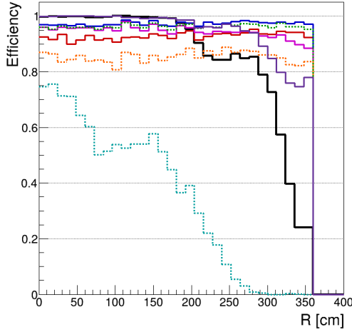
Figure 16: Single-photon efficiency without pileup for the exploratory CLUEstering configurations. The right panel shows 100\epsilon/\epsilon_{\text{CLUE3D}} ; 100 % denotes equal efficiency.
