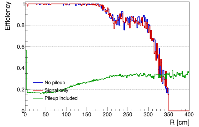
Figure 14: Default CLUE3D efficiency without pileup, for the generated signal photon in PU200, and for the inclusive in-time truth selection in PU200.
