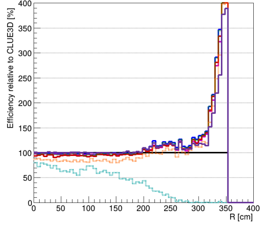
(a) Efficiency for the generated signal photon in PU200.
