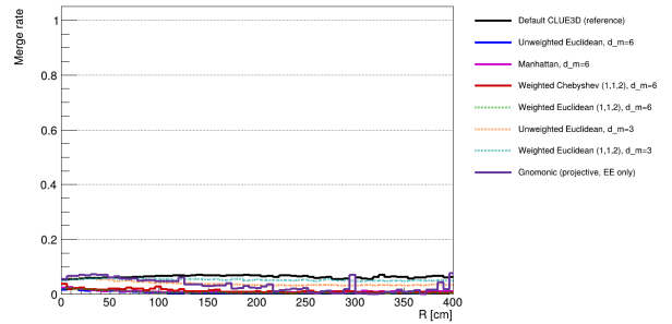
(b) Reconstructed-object merges versus barycentre radius.
