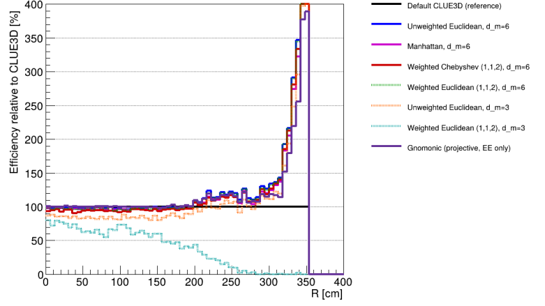
(a) Efficiency for the generated signal photon in PU200.
