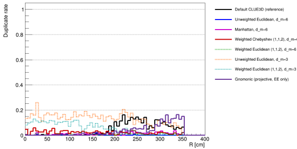
(a) Signal-photon duplicates versus truth displacement.
