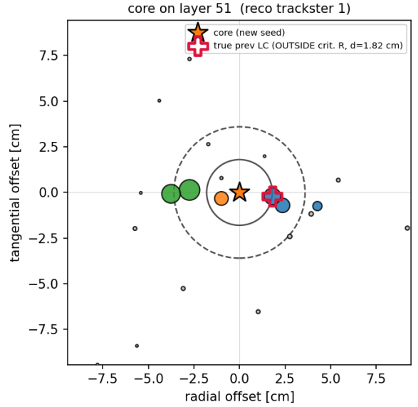
Figure 8: A neighbourhood in the full projected coordinates for the R \simeq 297 cm event previously shown in Fig. 7. The star marks the layer-51 core of a new fragment, and circles the 1.8 cm and 3.6 cm distances.
