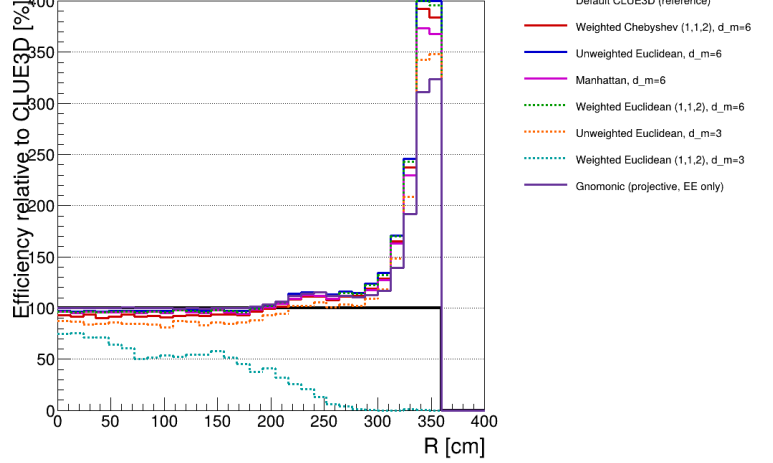
Figure 16: Single-photon efficiency without pileup for the exploratory CLUEsterng configurations. The right panel shows 100 \epsilon / \epsilon_{\text{CLUE3D}} ; 100 % denotes equal efficiency.
