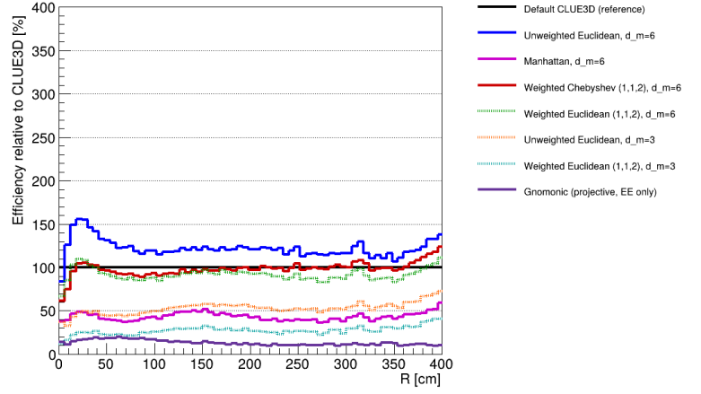
(b) Efficiency for the inclusive in-time truth population.
