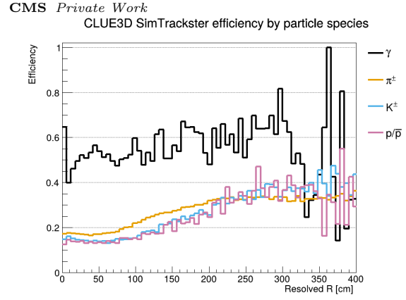
(b) Efficiency split by particle species.
