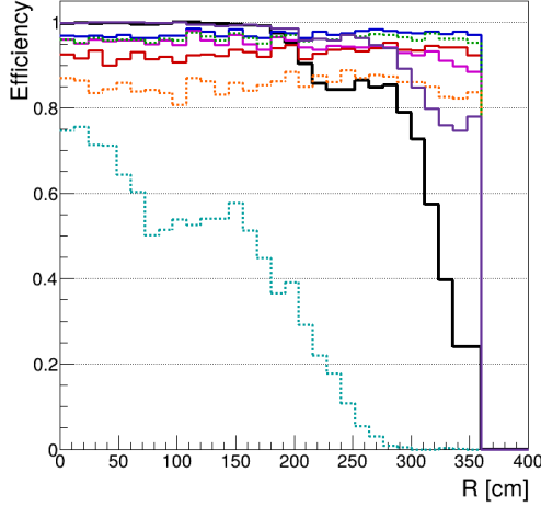
Figure 16: Single-photon efficiency without pileup for the exploratory CLUEsterng configurations. The right panel shows 100 \epsilon / \epsilon_{\text{CLUE3D}} ; 100 % denotes equal efficiency.
