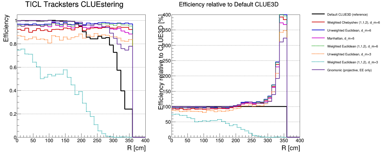
Figure 12: Single-photon efficiency without pileup for the exploratory CLUEsterng configurations. The right panel shows 100\epsilon/\epsilon_{\text{CLUE3D}} ; 100 % denotes equal efficiency.
