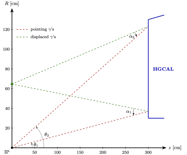
Figure 2: Displacement geometry in the (z, R) plane. Pointing photons (red) travel radially from the interaction point (IP) with \alpha = 0 ; displaced photons (green) originate at a transverse distance R from the beamline at z = 0 and hit the calorimeter with \alpha > 0 . The two green trajectories show that a single R can give different angles \alpha .
