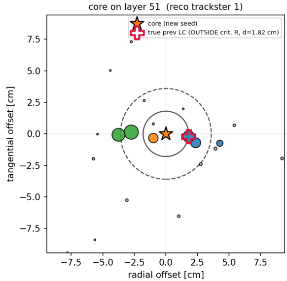
Figure 6: A neighbourhood in the full projected coordinates for the R \simeq 297 cm event. The star marks the layer-51 core of a new fragment, and circles the 1.8 cm and 3.6 cm distances.
