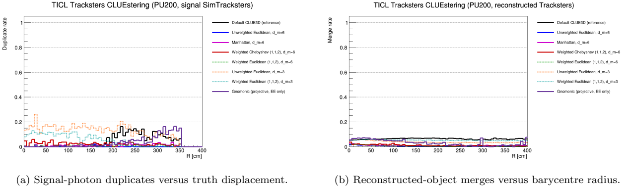
Figure 15: Complementary PU200 rates. The duplicate denominator contains signal SimTracksters, while the merge denominator contains reconstructed Tracksters.
