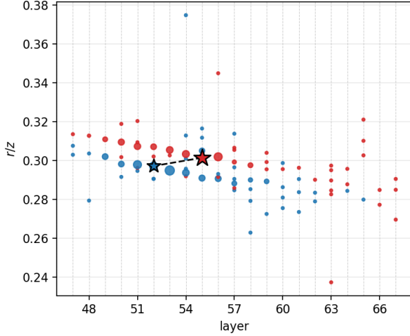
Figure 9: An actual cross-shower nearest-higher link for photons separated by s = 4 cm at R \simeq 131 cm, shown as r/z versus layer. Blue marks the shower A and red the other shower B ; the dashed line is the recorded nearest-higher hop from B 's highlighted LC (layer 55) to A 's (layer 52). The two lie at nearly the same r/z despite belonging to different showers.
