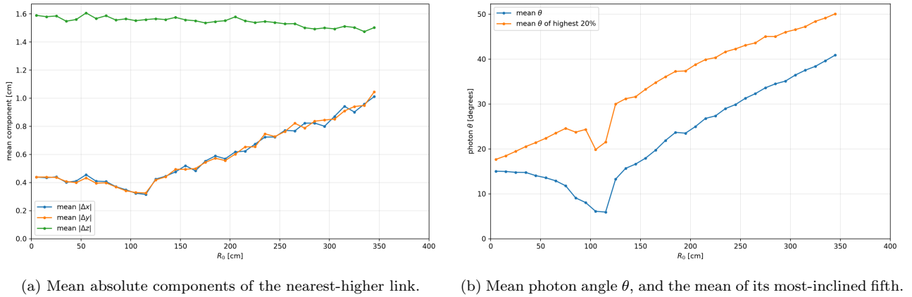
Figure 13: Diagnostics for the weighted Euclidean metric at d_m = 3 cm, versus truth displacement R_0 .
