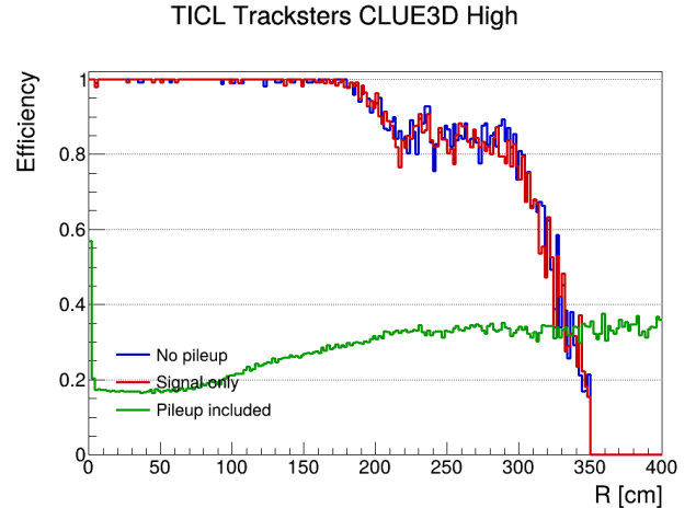
Figure 10: Default CLUE3D efficiency without pileup, for the generated signal photon in PU200, and for the inclusive in-time truth selection in PU200.
