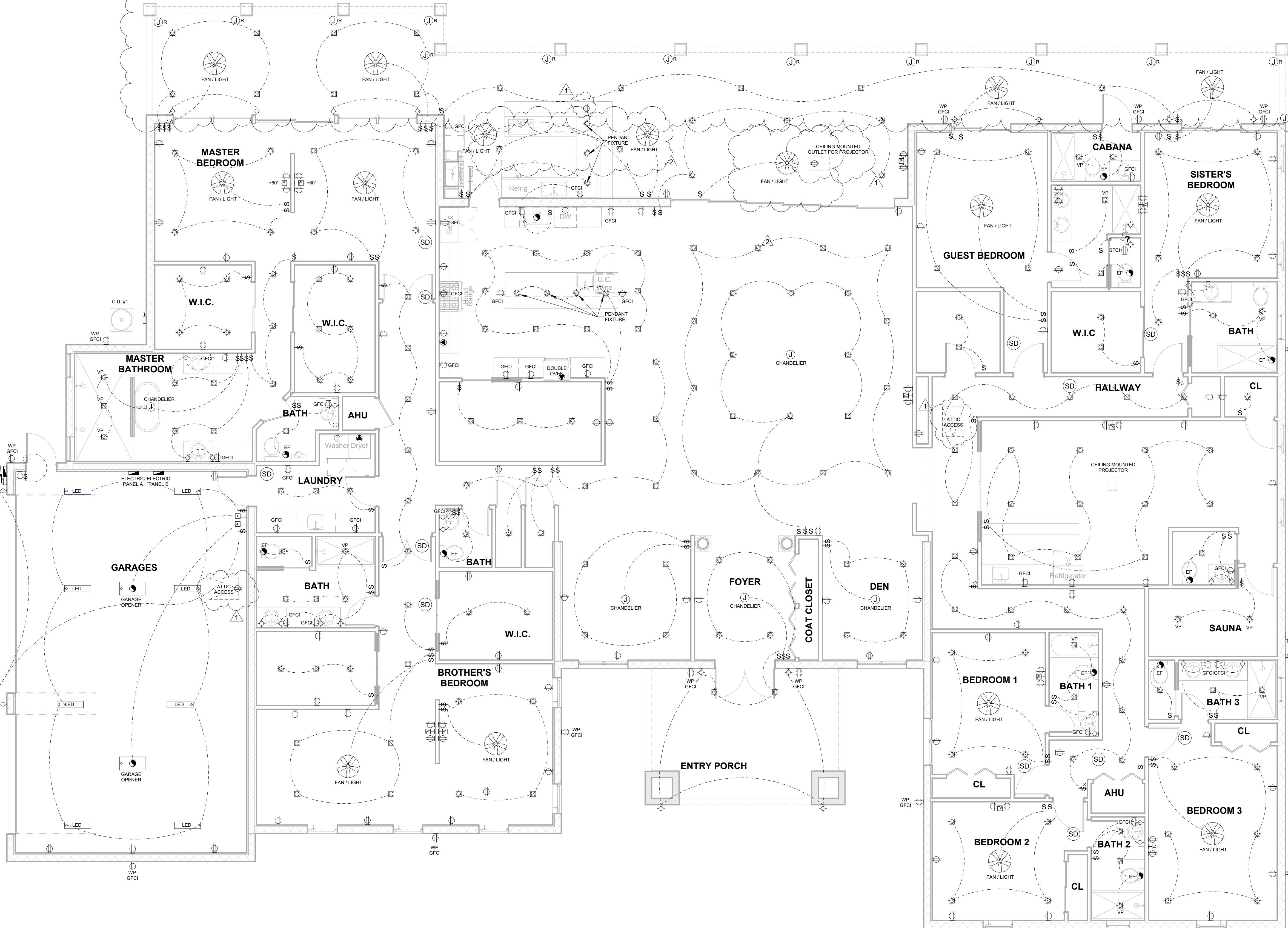
1 ELECTRICAL FLOOR PLAN 3/16" = 1'-0"
