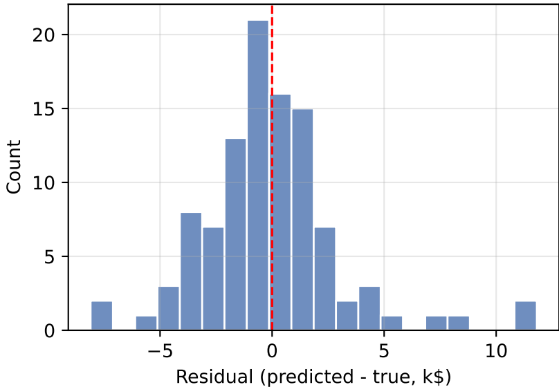
SVR-RBF test residuals
