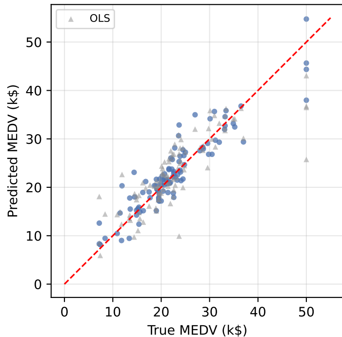
(b) Ridge+poly2 test: RMSE=3.24, R^2=0.851
