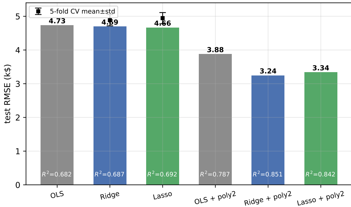
(a) Test RMSE of all models
