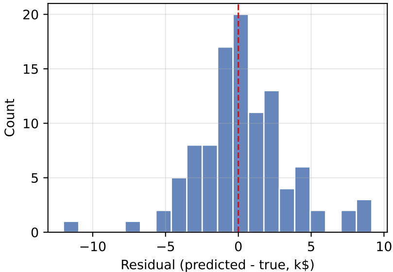
Ridge+poly2 test residuals
