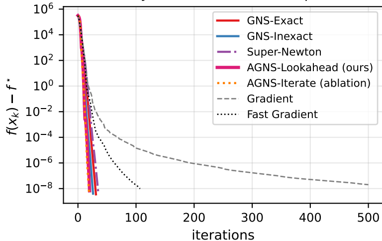
Chebyshev chain ( n=1000, p=4 )
