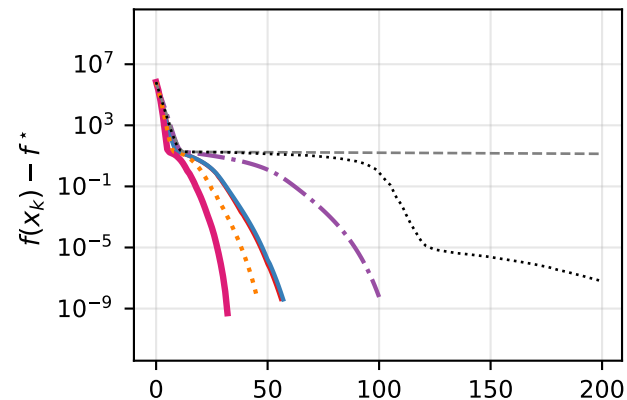
Rosenbrock-NLE p = 5
