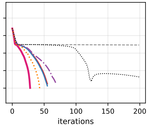
Rosenbrock-NLE p = 8
