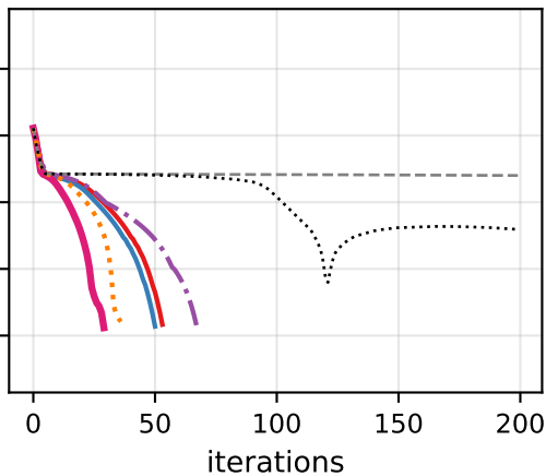
Rosenbrock-NLE p = 6
