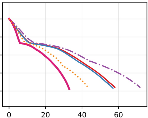
Rosenbrock-NLE p = 6
