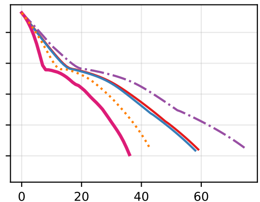
Rosenbrock-NLE p = 8
