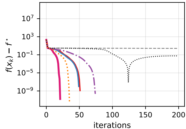
Rosenbrock-NLE p = 5
