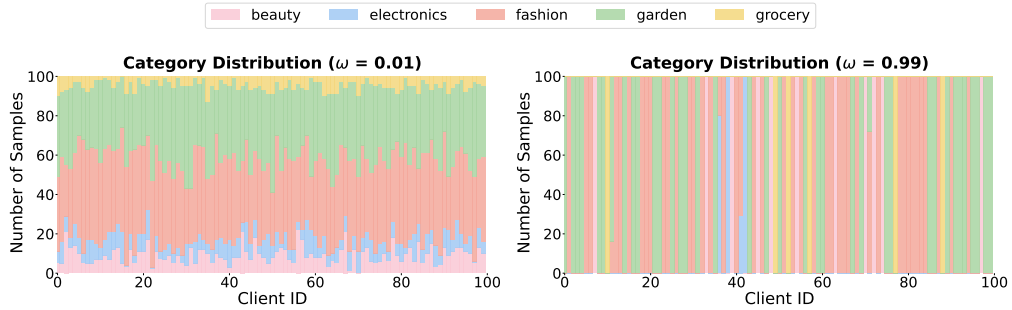
Figure 8: Client Distribution under Preference Heterogeneity (WebShop, \omega = 0.01 vs. \omega = 0.99 ). Each panel plots a client’s category histogram; the aggregate across clients recovers the global category marginal \pi , which is preserved between the two settings while the per-client spread grows sharply with \omega .
