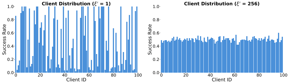
Figure 11: Client Distribution under Hardness Heterogeneity ( \xi' = 1 vs. \xi' = 256 ). Histograms show per-client success-rate quotas \rho_k . The per-client size and the global success rate are pinned, so only the spread changes. The same construction is applied identically to WebShop and ALFWorld.
