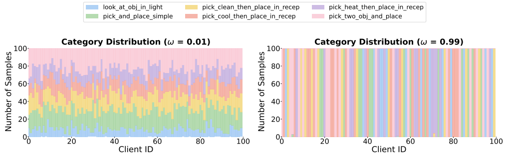
Figure 9: Client Distribution under Preference Heterogeneity (ALFWorld, \omega = 0.01 vs. \omega = 0.99 ). The six household task types (e.g., pick & place , clean & place ) play the role of categories. Per-client concentration grows sharply with \omega while the aggregate marginal stays fixed.
