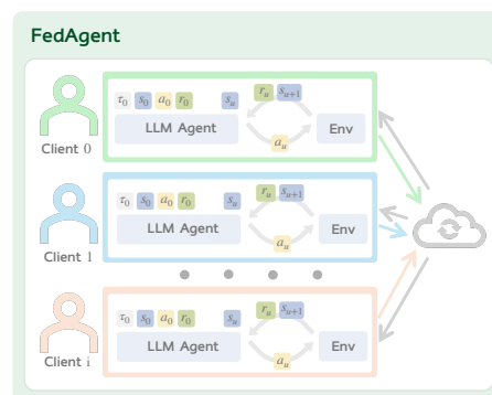
Figure 1: An Illustration for FEDAGENT.
