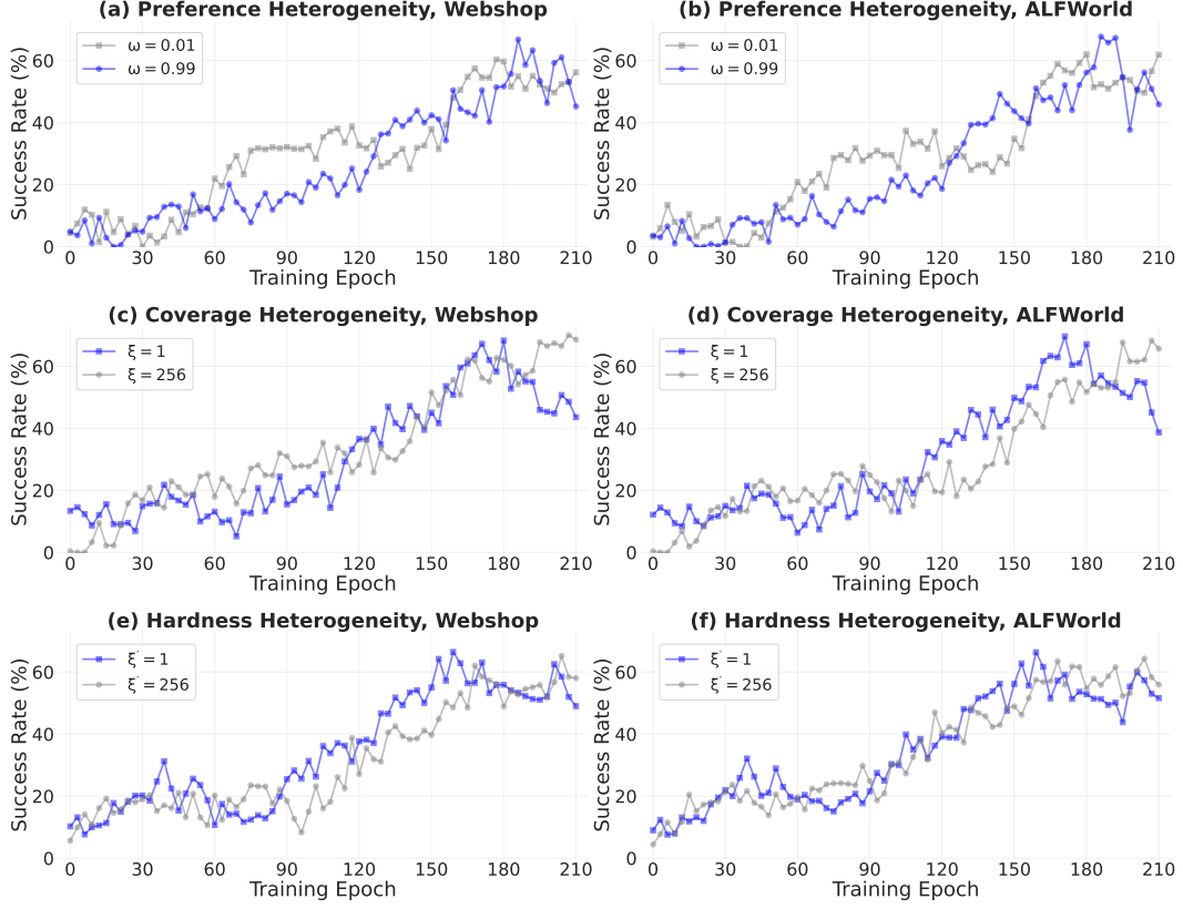
Figure 7: Training dynamics of FEDAGENT (PPO) under task-level heterogeneity , counterpart of Figure 4. The federated curve under extreme task heterogeneity (blue) matches the near-uniform baseline (grey) at the final plateau across all three sub-types (preference, coverage, hardness) and both benchmarks (WebShop, ALFWorld), with a transient slow-start under extreme hardness ( \xi'=1 , panels e, f) before catching up by epoch \sim 90 , confirming Pattern A also holds under PPO.
