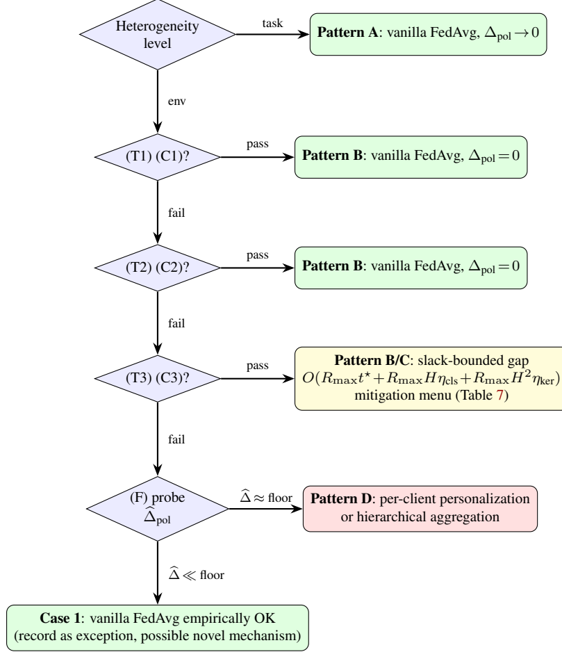
Figure 12: Mitigation decision tree for federated agent deployments. Diamonds are tests defined in §M.8.1 (T1, T2, T3) and §M.8.4 (F); rectangles are outcomes paired with the structural mitigation. Tests are evaluated sequentially top-to-bottom on a small probe rollout; the first passing test exits to the right with a vanilla-FedAvg or slack-bounded prescription. The empirical probe (F) at the bottom resolves the (C1)-(C3)-fail case into either Pattern D (personalization required, red) or Case 1 (vanilla FedAvg empirically adequate, green); “floor” here refers to the worst-case lower bound \Omega(R_{\max} H \delta) of Theorem 4. Color coding: green = \Delta_{\text{pol}} = 0 or \rightarrow 0 ; yellow = bounded but nonzero gap; red = structural floor binds.
