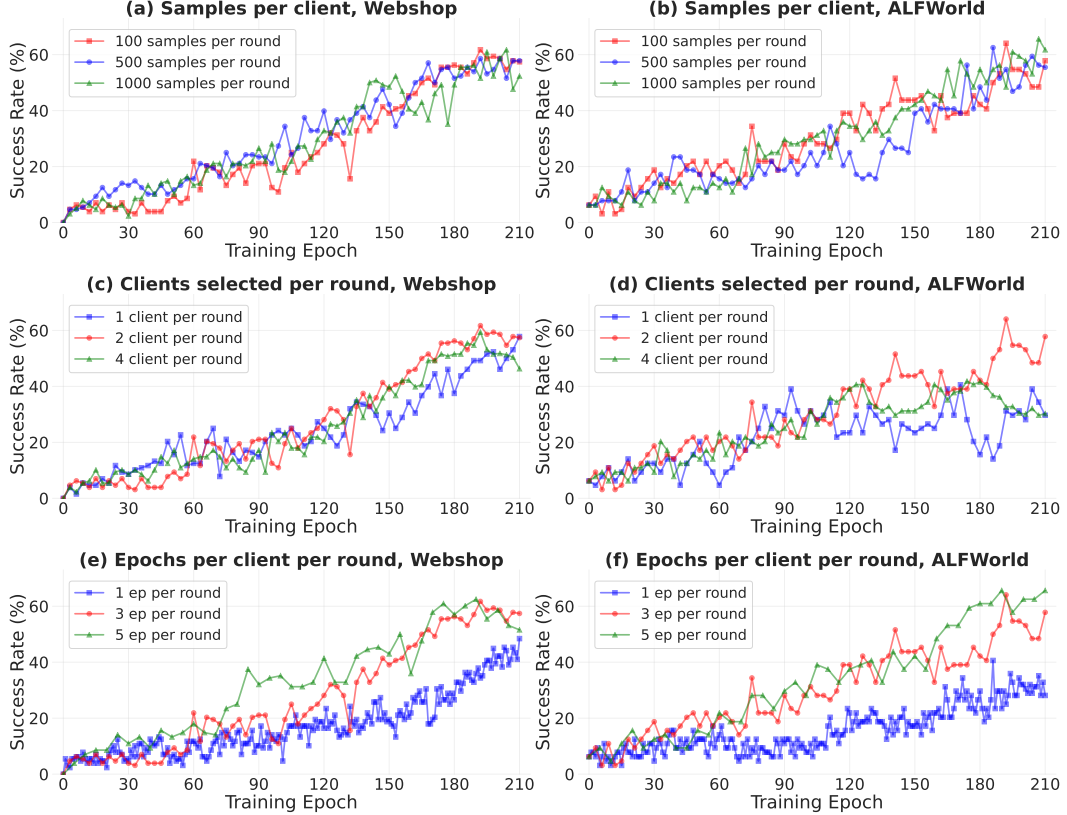
Figure 6: Sensitivity of FEDAGENT to federated configuration hyperparameters on WebShop and ALFWorld. Across the sweep over (|X_i|, M, E) , only E and M affect final performance meaningfully; |X_i| saturates above \sim 100 .
