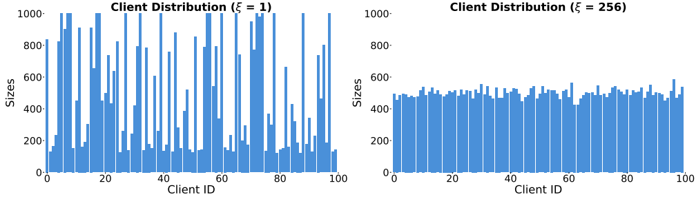
Figure 10: Client Distribution under Coverage Heterogeneity ( \xi = 1 vs. \xi = 256 ). Histograms show per-client pool sizes \{n_k\} . The per-client mean and the global replica budget are pinned across the two settings, so only the spread changes. The same construction is applied identically to WebShop and ALFWorld.
