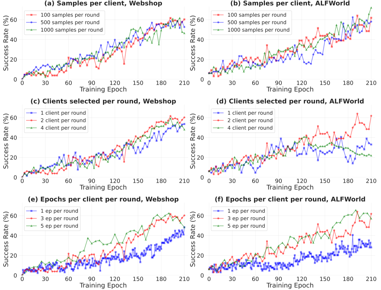
Figure 6 | Sensitivity of FEDAGENT to federated configuration hyperparameters on WebShop and ALFWorld. Across the sweep over (|X_i|, M, E) , only E and M affect final performance meaningfully; |X_i| saturates above \sim 100 .
