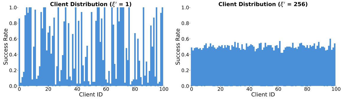
Figure 11 | Client Distribution under Hardness Heterogeneity ( \xi' = 1 vs. \xi' = 256 ). Histograms show per-client success-rate quotas \rho_k . The per-client size and the global success rate are pinned, so only the spread changes. The same construction is applied identically to WebShop and ALFWorld.
