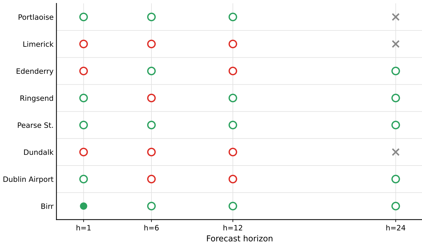
Diebold-Mariano test: lags+met vs lags only — Ireland PM10, 2023 (Global BH across 33 valid tests)
