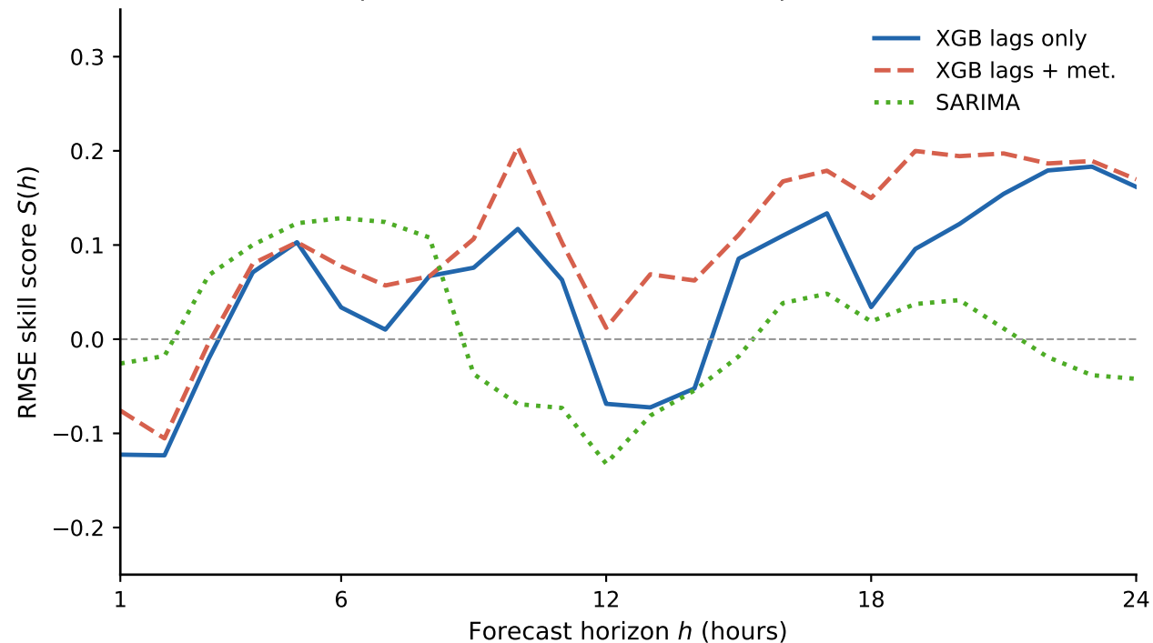
Forecast skill comparison — Madrid Casa de Campo PM10
