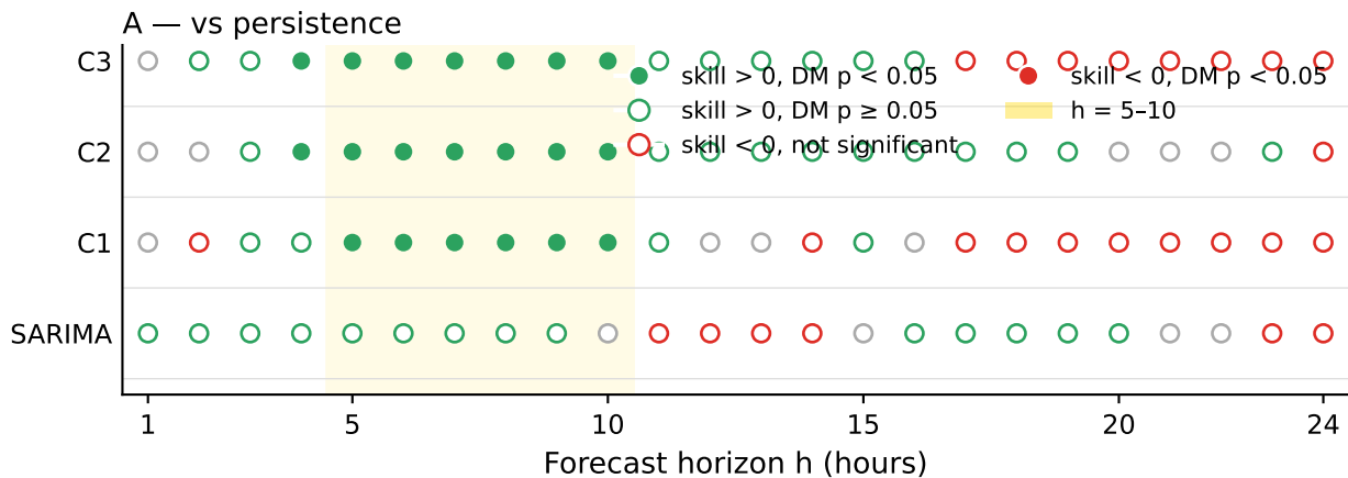
DM significance panel — Madrid station 24, 2023
