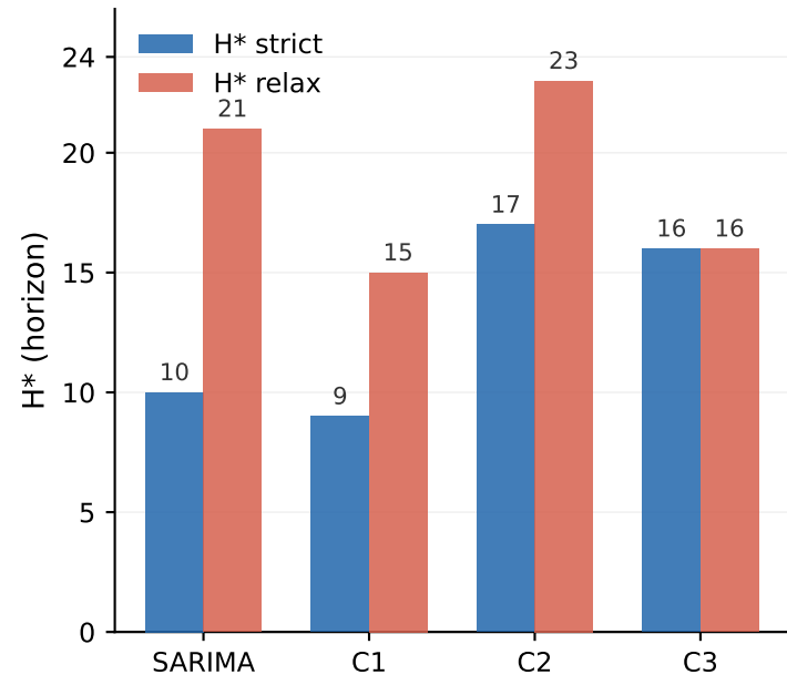
A — vs persistence
