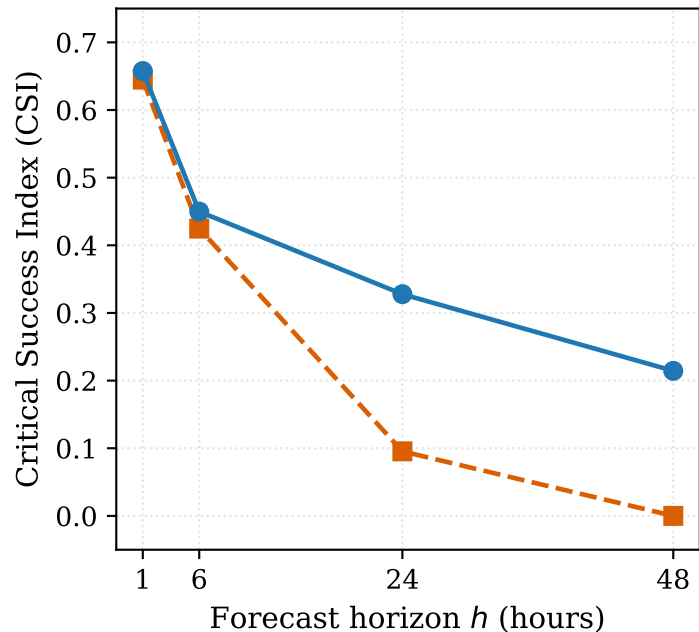
(c) Event Detection (CSI at p_{75} )
