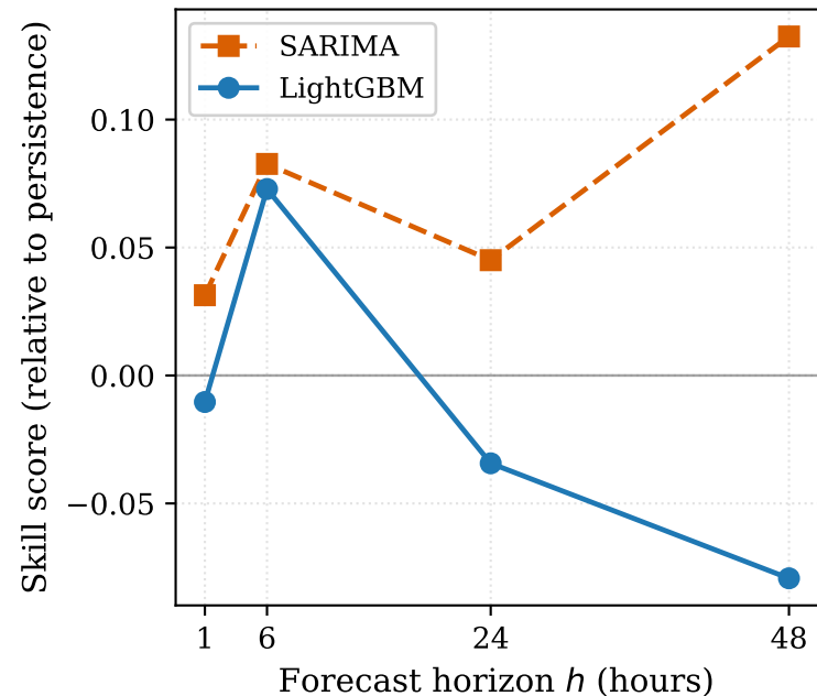
(a) RMSE Skill ( 1 - \text{RMSE}/\text{RMSE}_{\text{pers}} )
