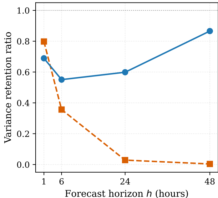
(b) Variance Retention ( \text{Var}(\hat{y})/\text{Var}(y) )
