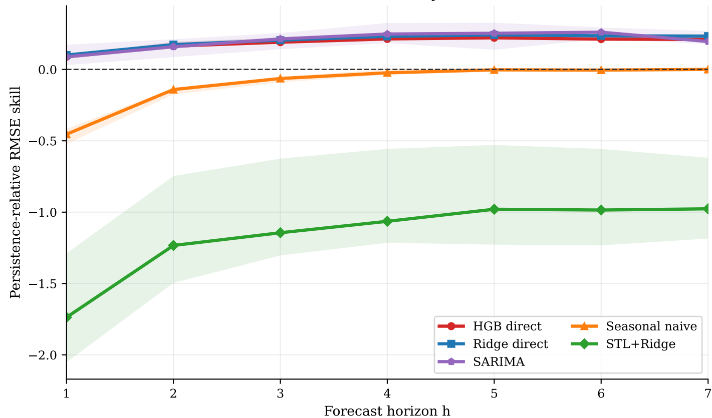
Median RMSE skill by horizon
