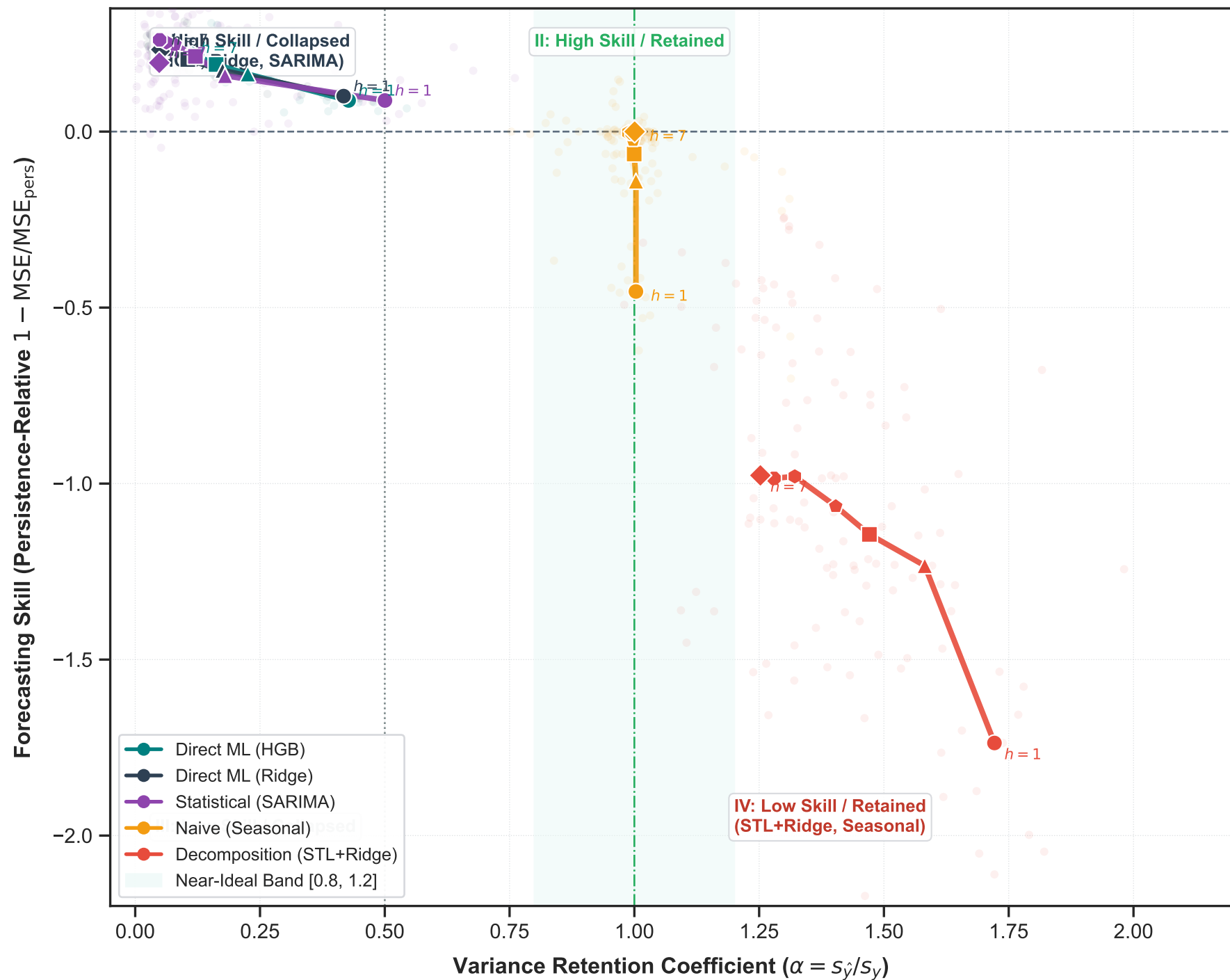
The Predictability-Variance Frontier in PM10 Forecasting
