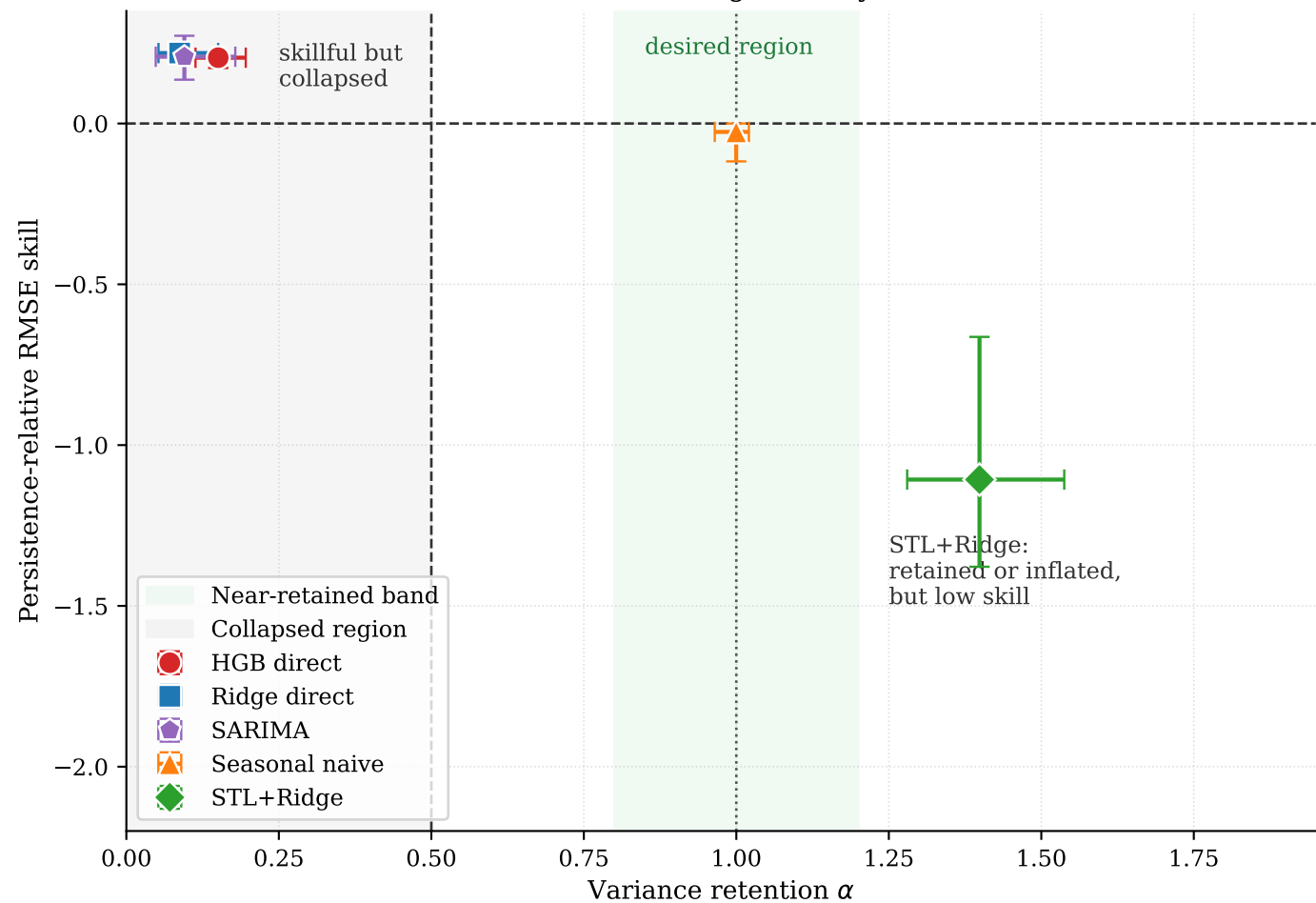
Skill-retention diagnostic by model
