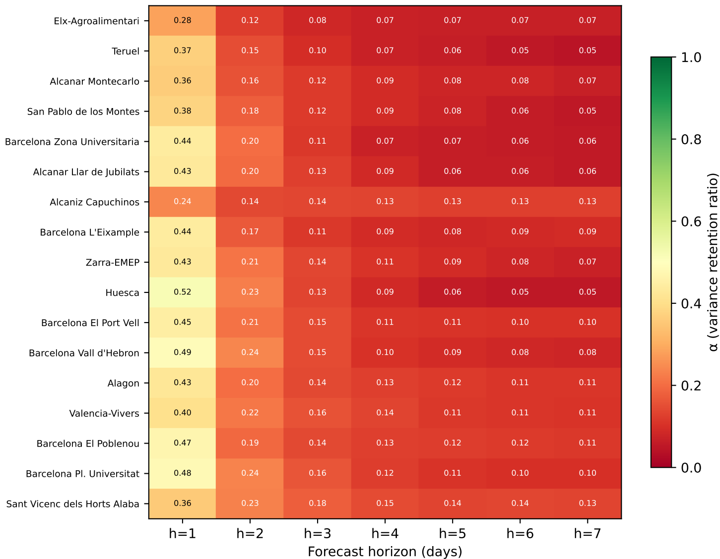
Variance retention ratio ( \alpha ) — Direct ML models (station \times horizon median)
