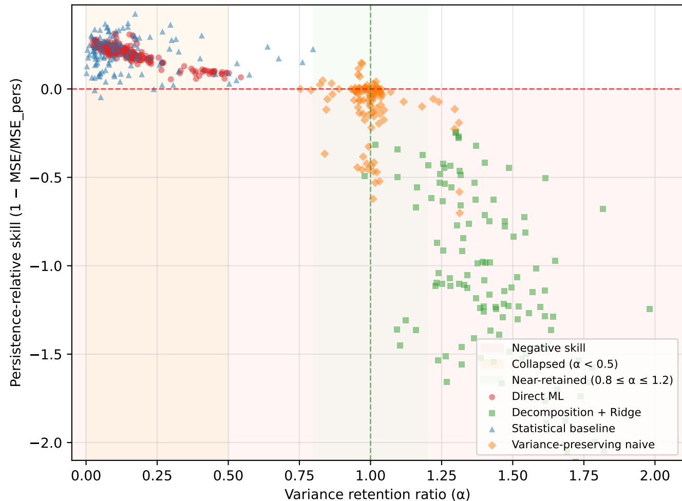
Skill vs. variance retention — all model \times station \times horizon cells
