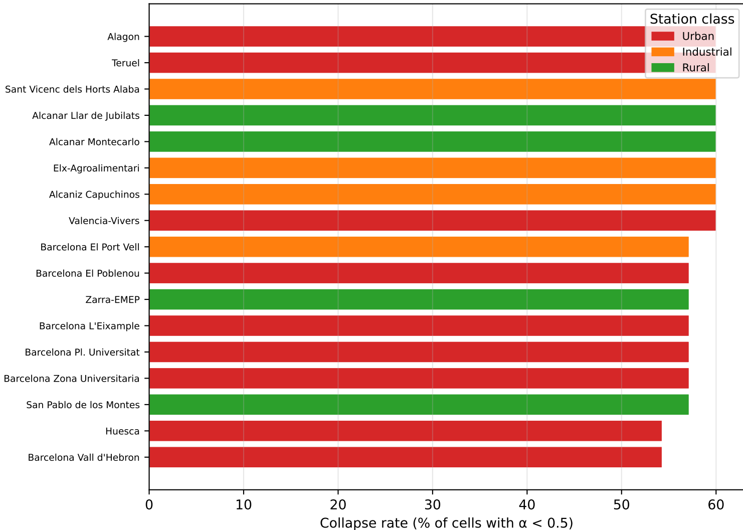
Station-level variance collapse rates (all models \times horizons)
