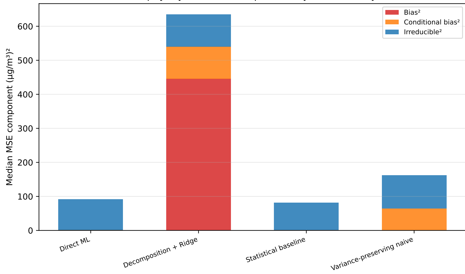
Murphy-style MSE decomposition by model family
