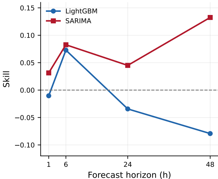
(A) Persistence-relative RMSE skill
