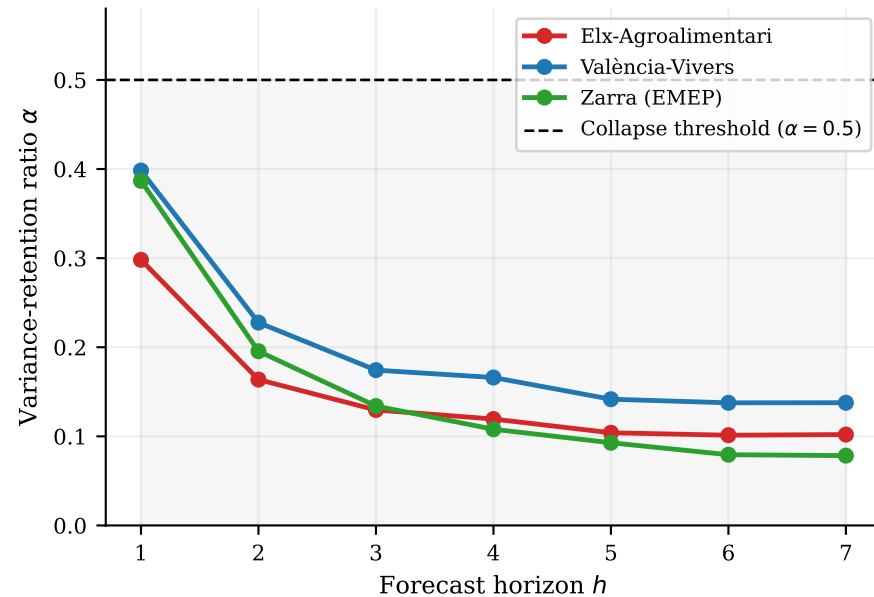
model: hgb_direct
