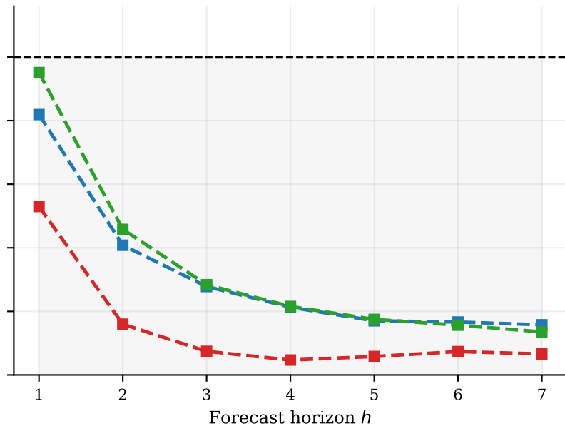
model: ridge_direct
