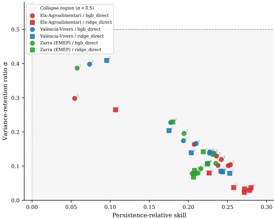
Skill-variance retention: all 42 model/station/horizon cells
