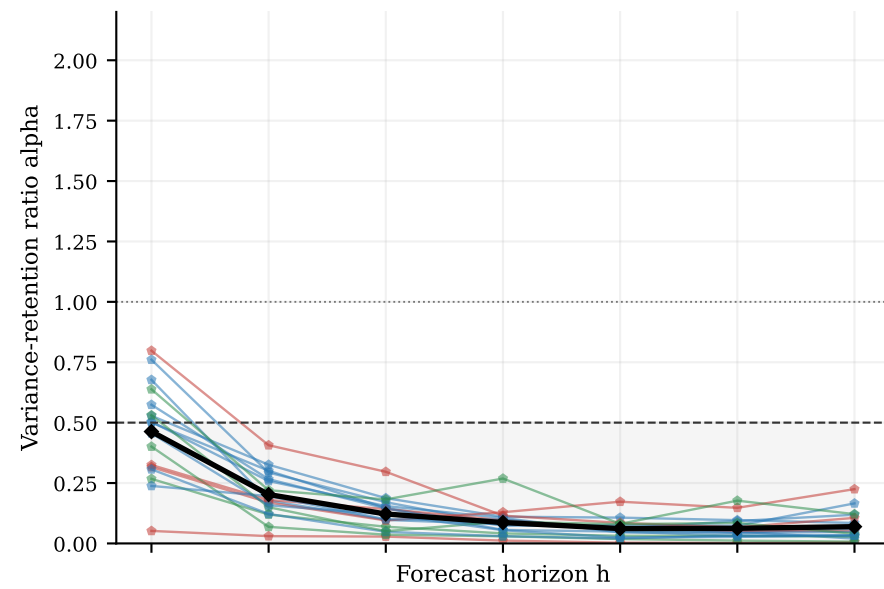
STL+Ridge
