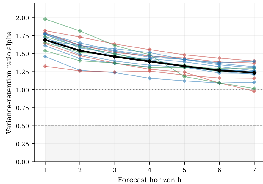
STL+Ridge
