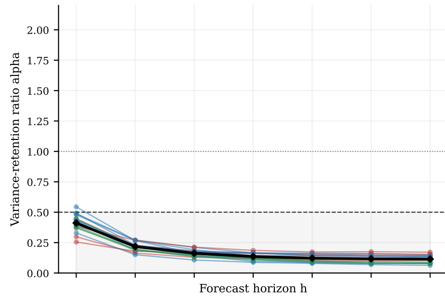
SARIMA
