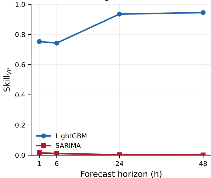
(C) Diagnostic Skill VP
