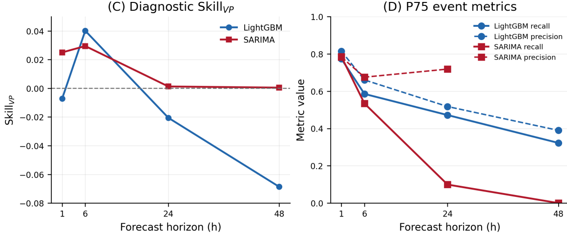
Figure 2: Diagnostic complements for horizon-wise interpretation. Left : Skill VP , which adjusts persistence-relative RMSE skill by variance retention. Right : horizon-wise exceedance recall and precision at the P75 threshold under fold-recalibrated evaluation.
