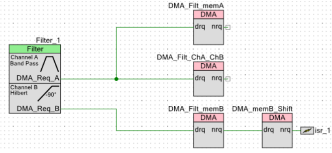
Fig. 7: Digital filters implemented in hardware after signal digitization for in-phase and quadrature component extraction.
