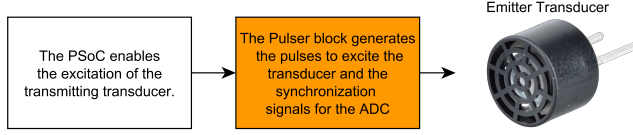
Fig. 3: Block diagram illustrating the transducer excitation procedure. Hardware-implemented operations are shown in orange, while software-controlled processes are shown in white.
