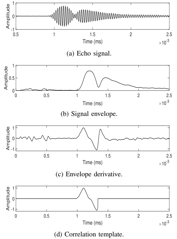
Fig. 2: Processing sequence for the correlation of the echo envelope derivative (CEED) method: (a) echo signal with destructive interference, (b) signal envelope, (c) envelope derivative, and (d) correlation template.
